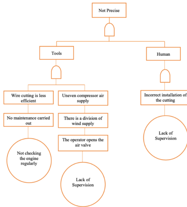
Figure 6. Fault Tree Analysis Not Precise
